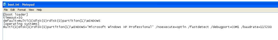
Figure 3: Change boot.ini settings
